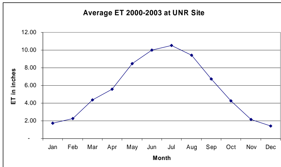
Figure 7-3 Monthly ET Rates
